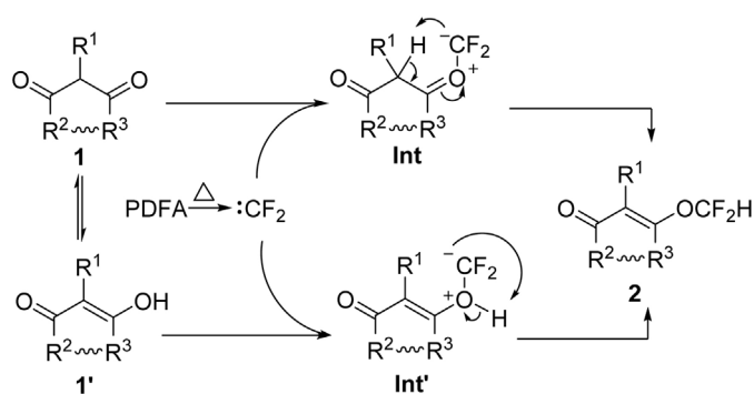
Scheme 2. The plausible reaction mechanism.
