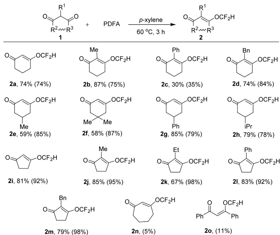
Scheme 1. Substrate scope for O -difluoromethylation. Isolated yields. Values in parentheses are the yields determined by 19 F NMR.
